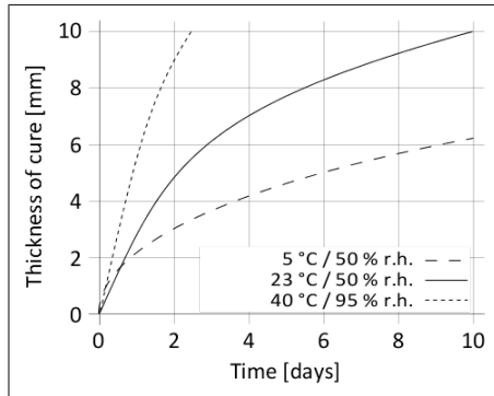
Diagram 1: Curing speed Sikasil® SG-20 S
